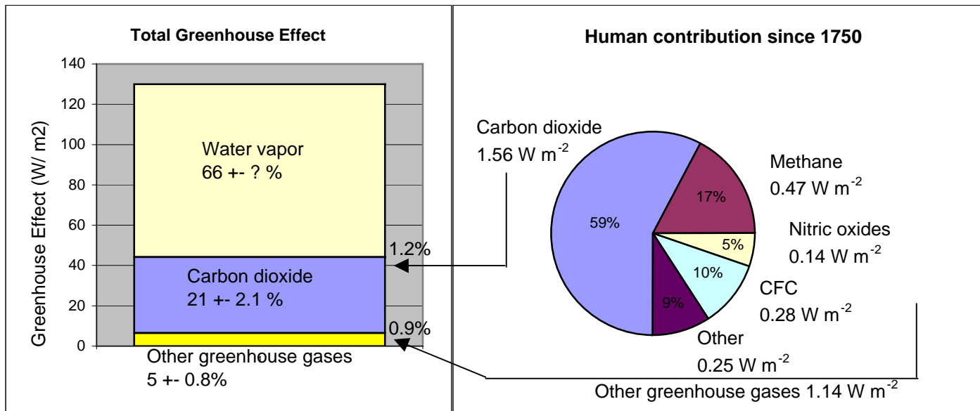
Figure 4.21: Water vapor is the most relevant greenhouse gas in the atmosphere, followed by carbon dioxide and the other trace gases ozone, methane, and nitric oxide. The anthropogenic contribution to this greenhouse system amounts to approximately 2.7 W / m^2 or 2.1%.
